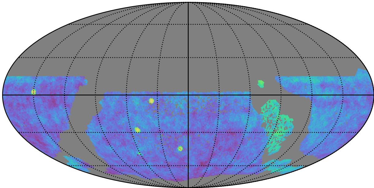
ddf_half_v3.4_10yrs gri WFD: Fraction of visits in pairs (10-60 min)
