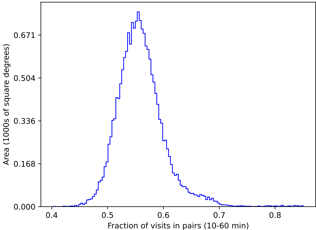
ddf_half_v3.4_10yrs gri WFD: Fraction of visits in pairs (10-60 min)
