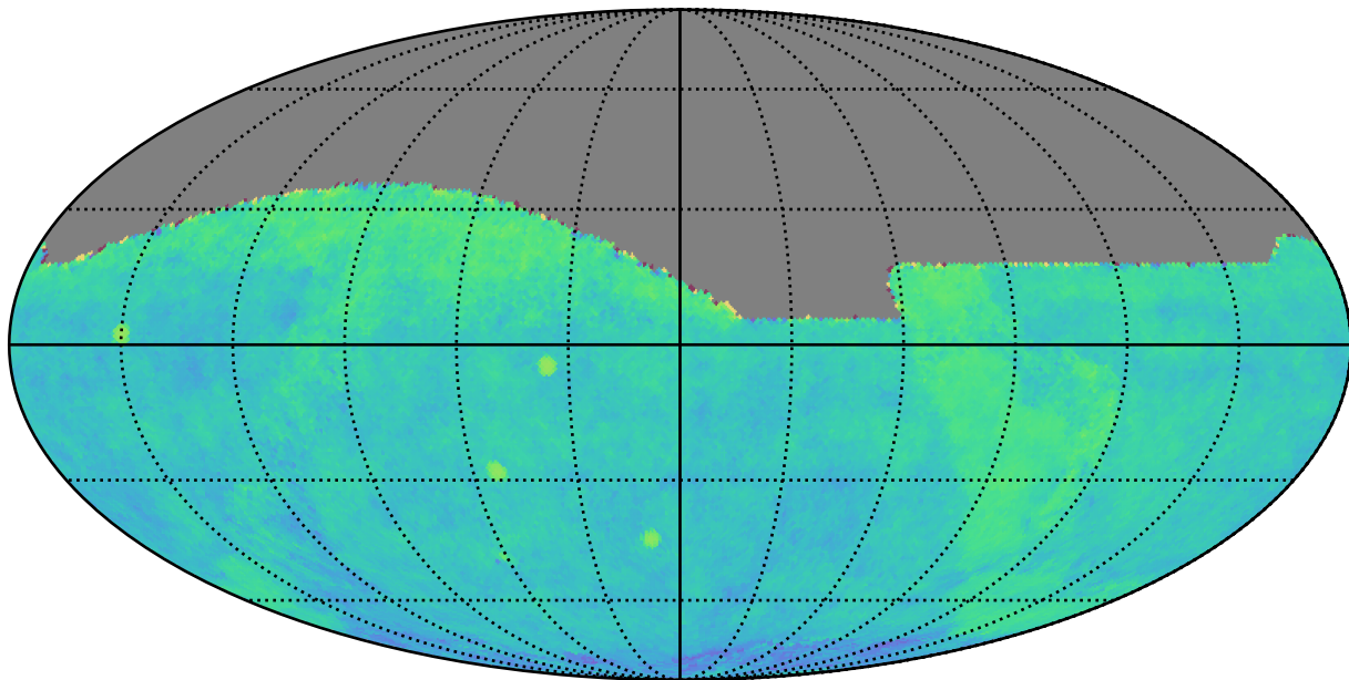
ddf_half_v3.4_10yrs gri All sky: Fraction of visits in pairs (10-60 min)
