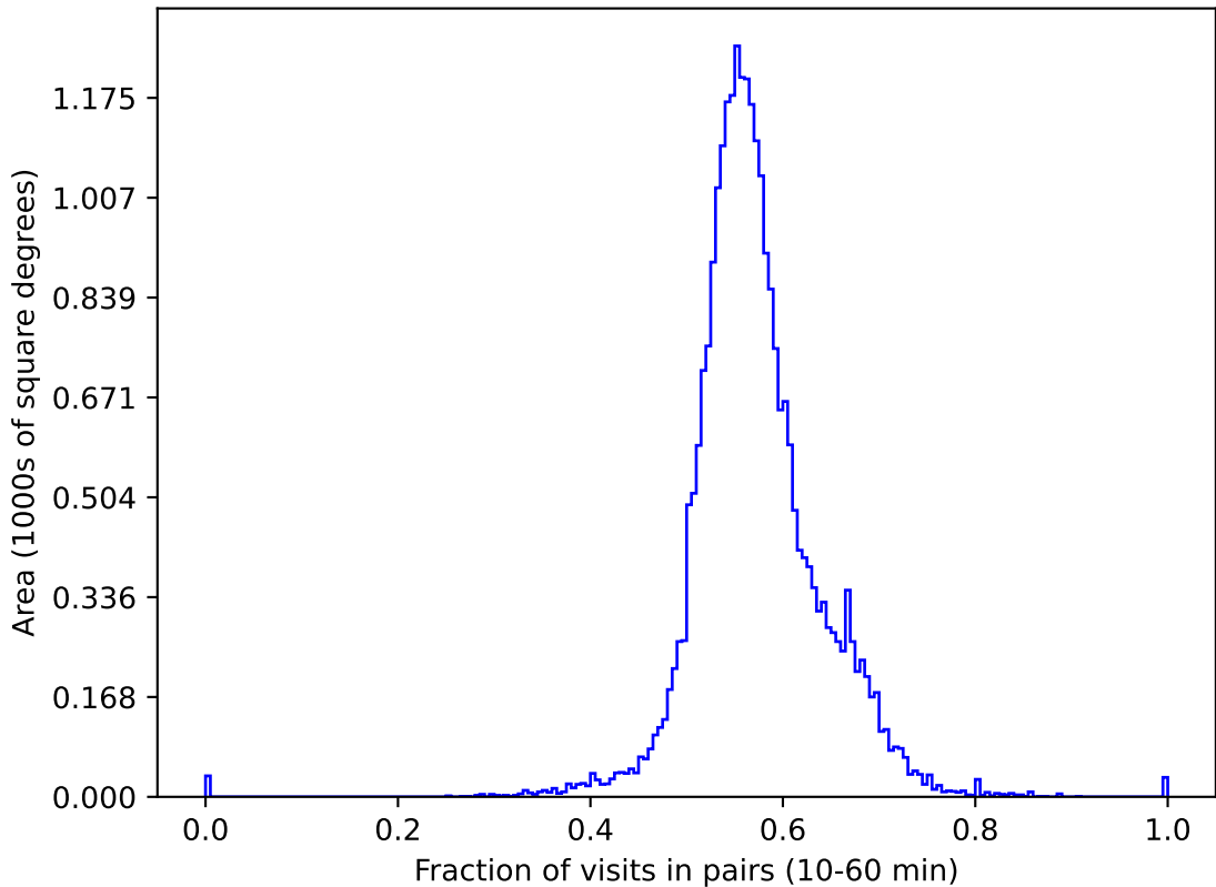
ddf_half_v3.4_10yrs gri All sky: Fraction of visits in pairs (10-60 min)
