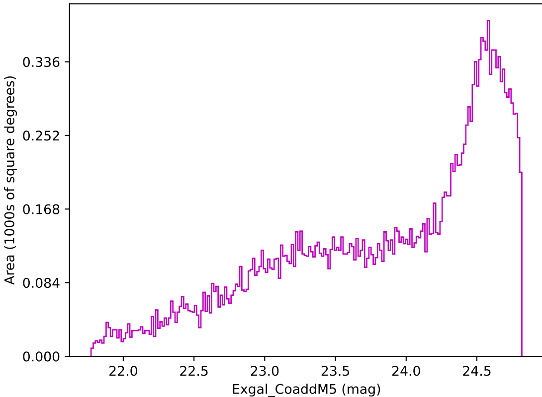
ddf_half_v3.4_10yrs Yr 3-4 z band: Exgal_CoaddM5
