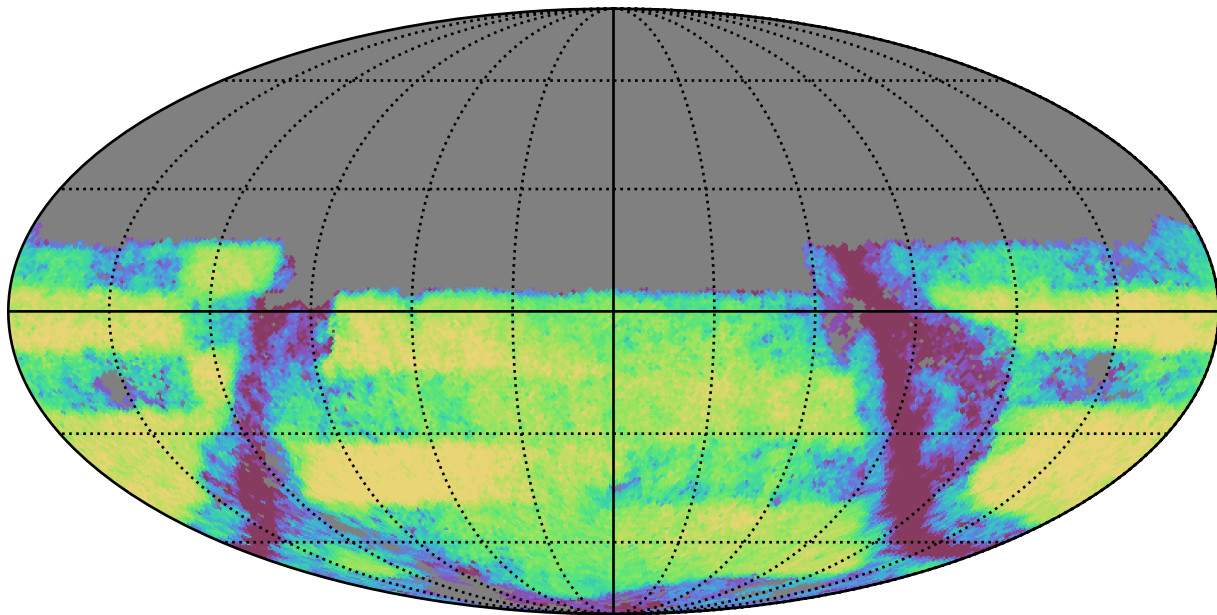
ddf_half_v3.4_10yrs Yr 3-4 y band: Exgal_CoaddM5
