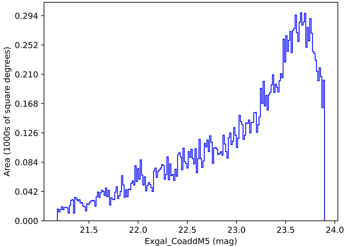
ddf_half_v3.4_10yrs Yr 3-4 y band: Exgal_CoaddM5
