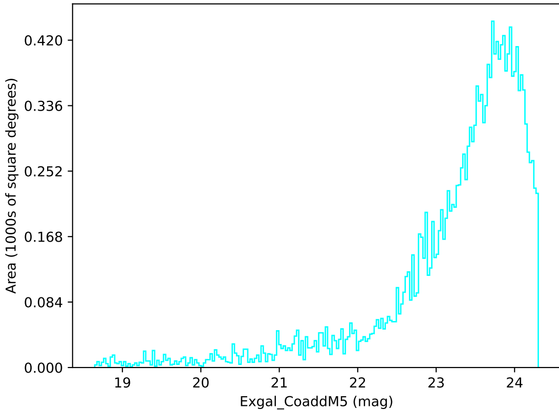
ddf_half_v3.4_10yrs Yr 3-4 u band: Exgal_CoaddM5
