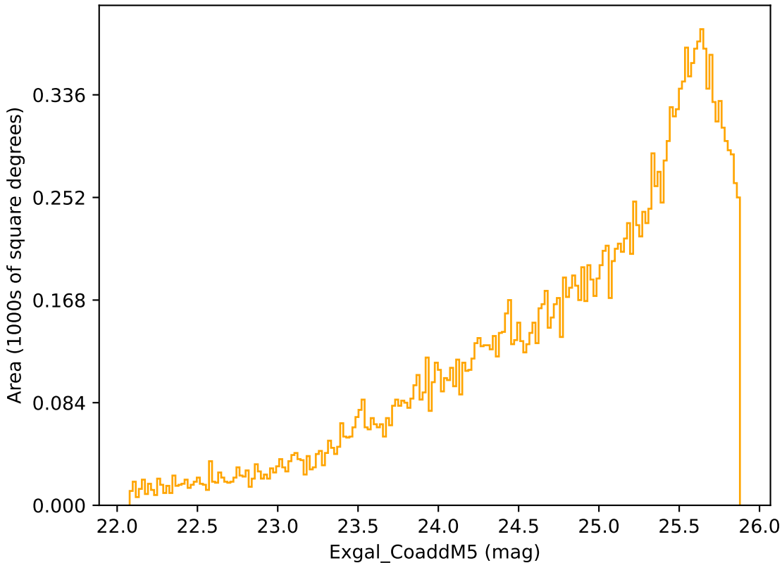
ddf_half_v3.4_10yrs Yr 3-4 r band: Exgal_CoaddM5
