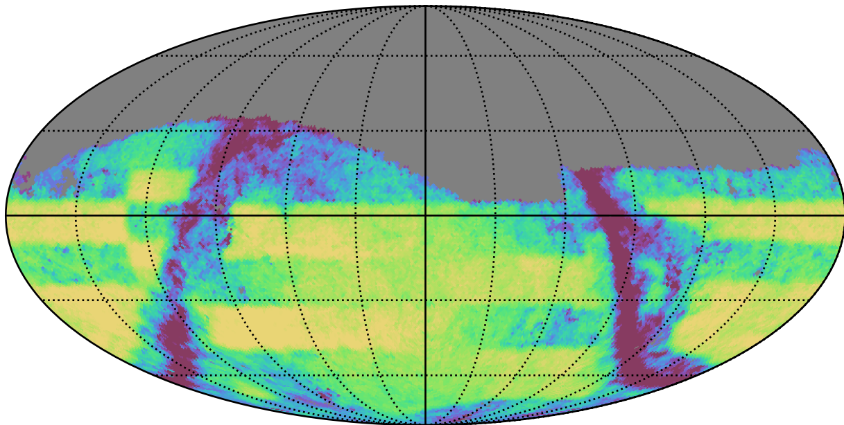
ddf_half_v3.4_10yrs Yr 3-4 i band: Exgal_CoaddM5
