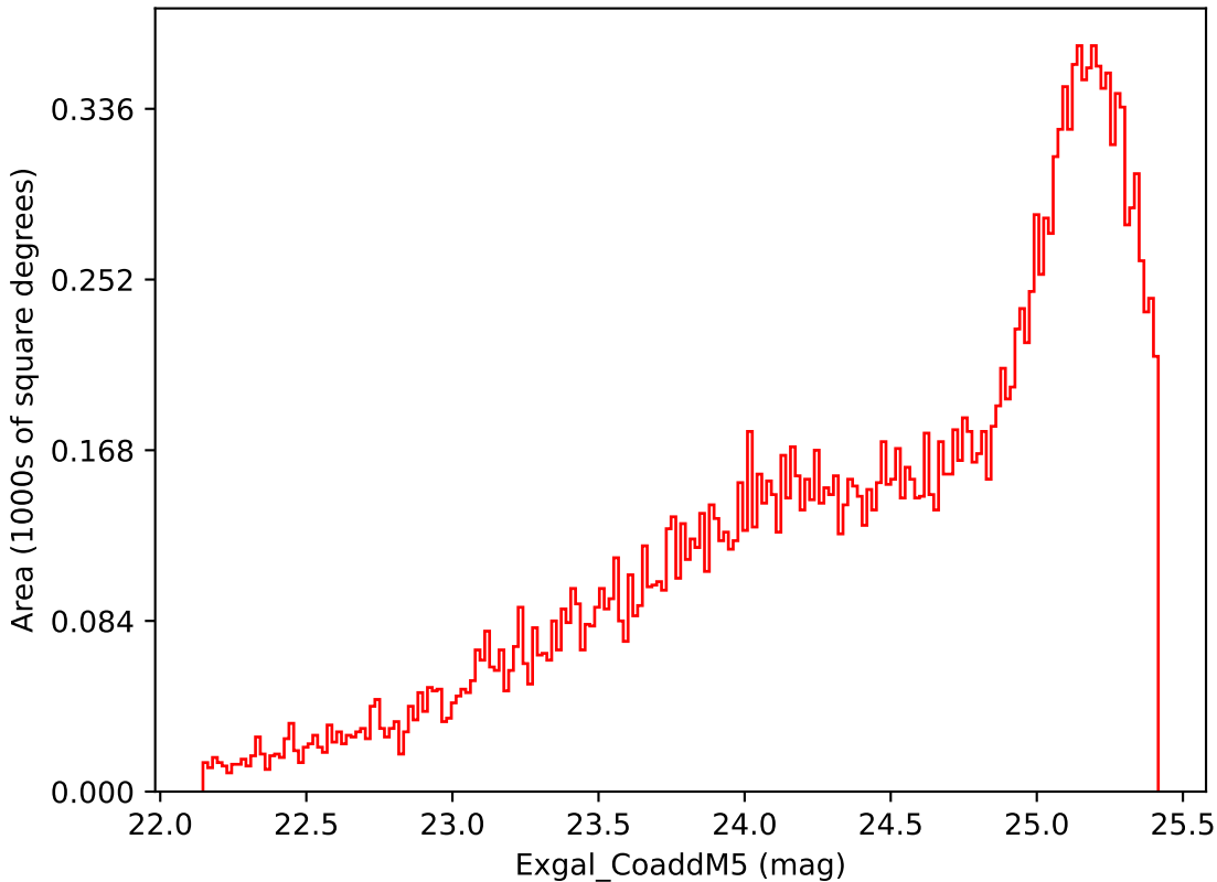
ddf_half_v3.4_10yrs Yr 3-4 i band: Exgal_CoaddM5
