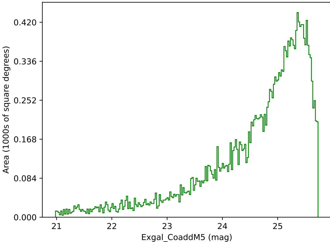
ddf_half_v3.4_10yrs Yr 3-4 g band: Exgal_CoaddM5
