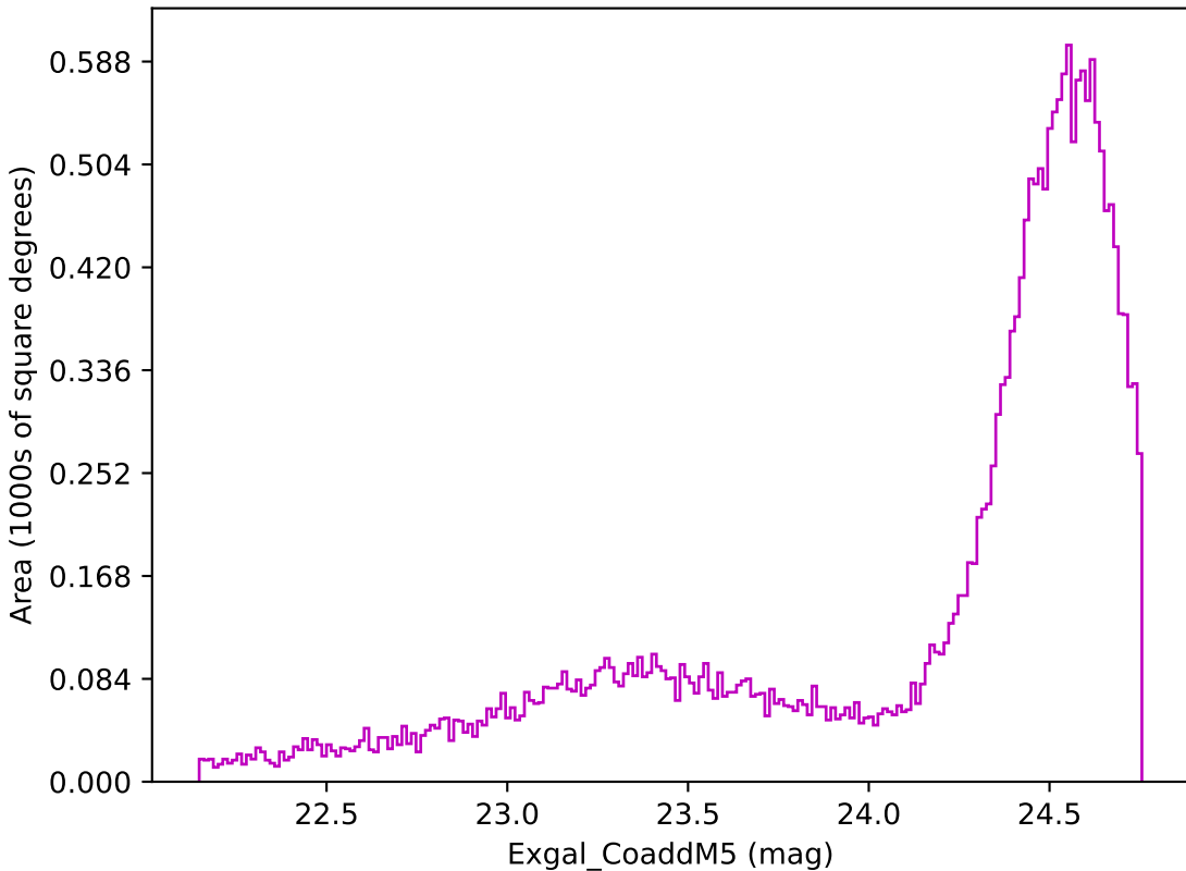
ddf_half_v3.4_10yrs Yr 1 z band: Exgal_CoaddM5
