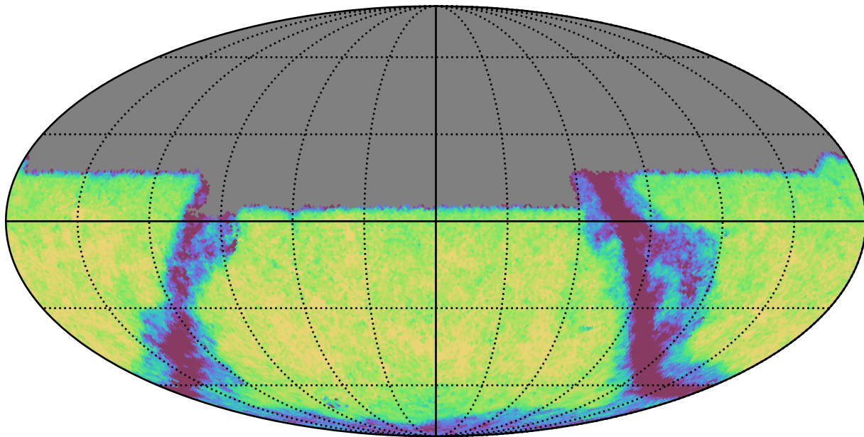
ddf_half_v3.4_10yrs Yr 1 y band: Exgal_CoaddM5
