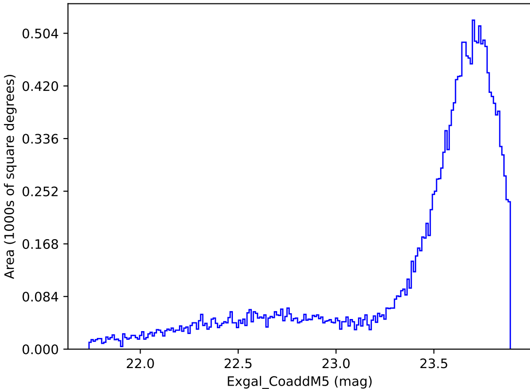
ddf_half_v3.4_10yrs Yr 1 y band: Exgal_CoaddM5
