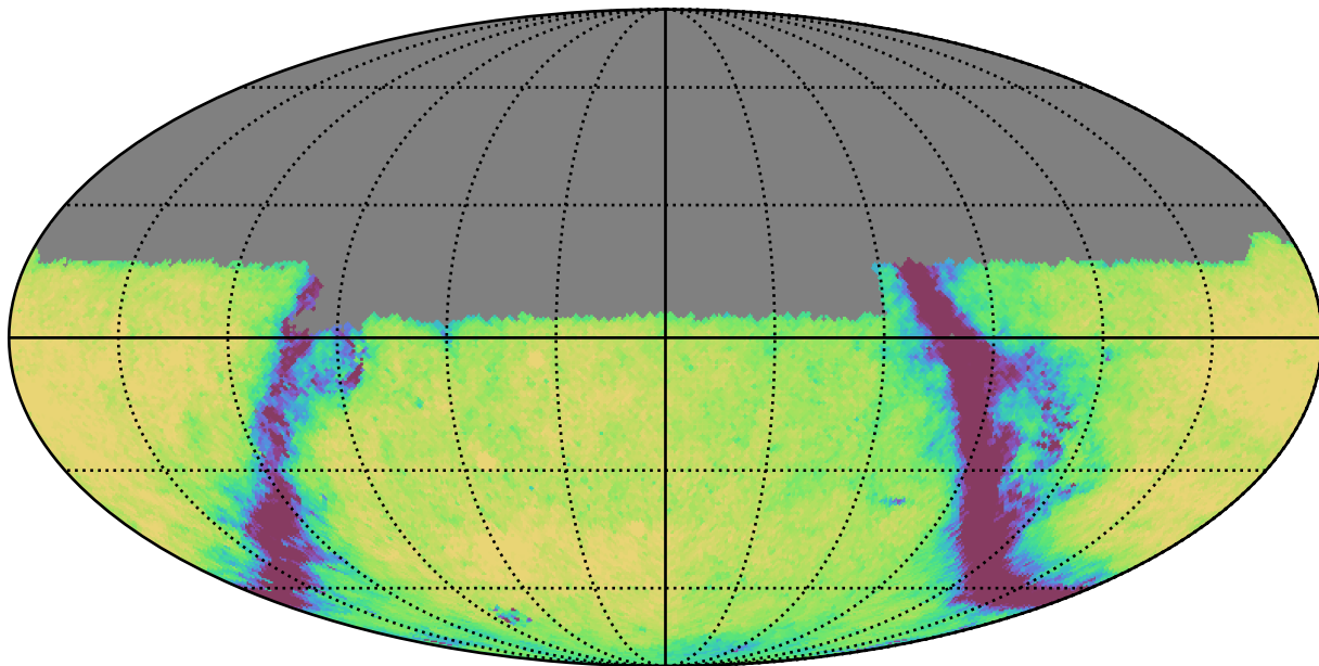
ddf_half_v3.4_10yrs Yr 1 u band: Exgal_CoaddM5
