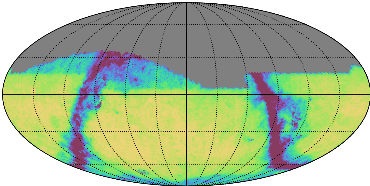
ddf_half_v3.4_10yrs Yr 1 r band: Exgal_CoaddM5
