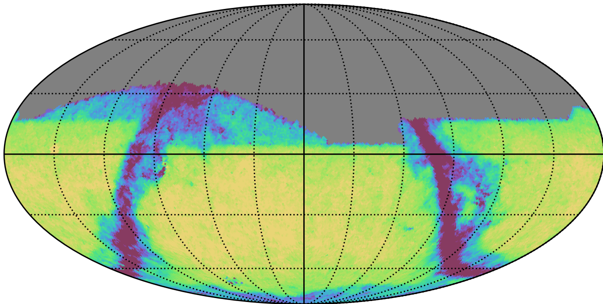
ddf_half_v3.4_10yrs Yr 1 i band: Exgal_CoaddM5
