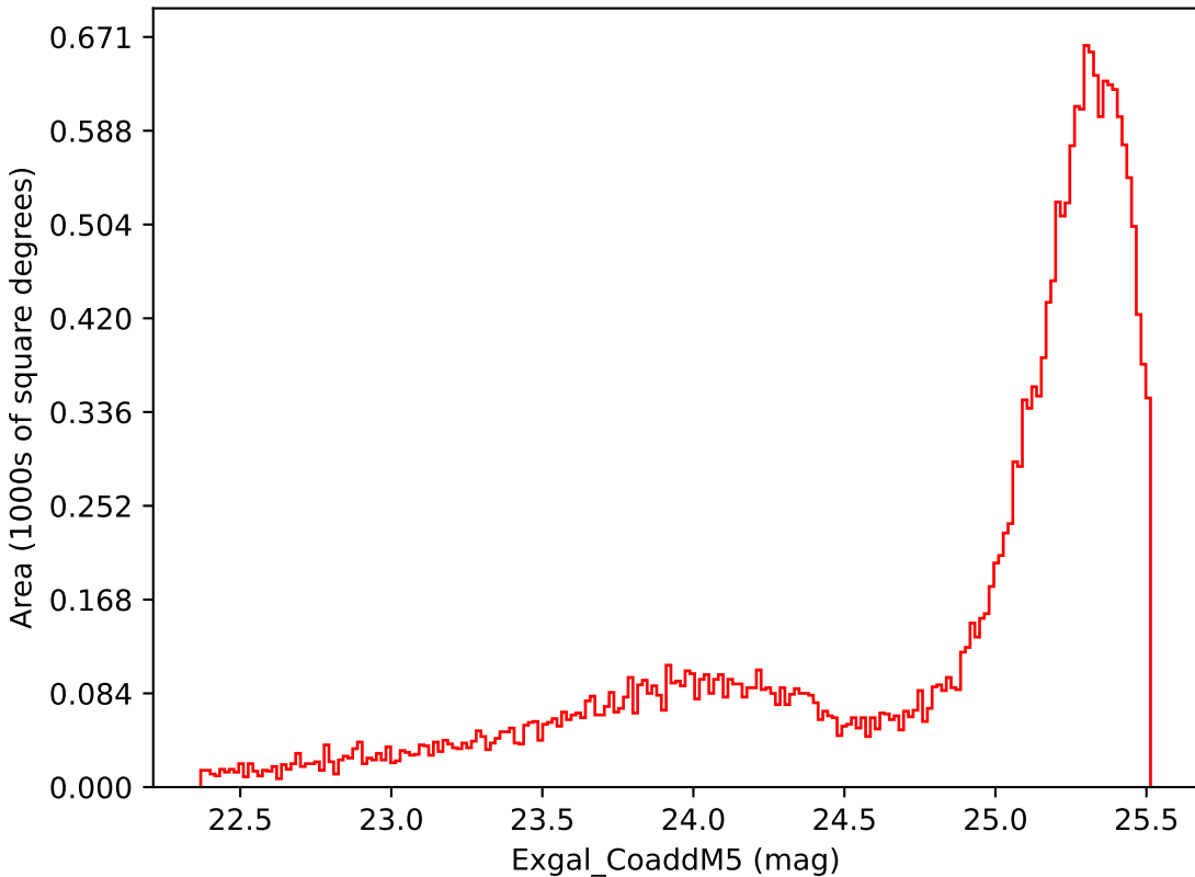
ddf_half_v3.4_10yrs Yr 1 i band: Exgal_CoaddM5
