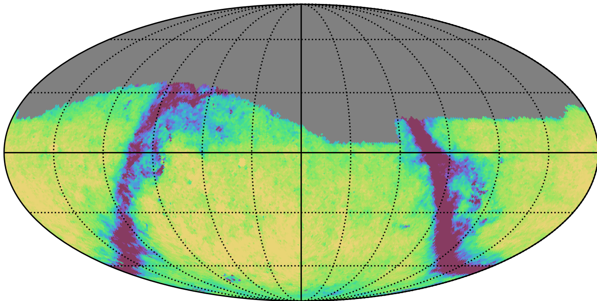
ddf_half_v3.4_10yrs Yr 1 g band: Exgal_CoaddM5
