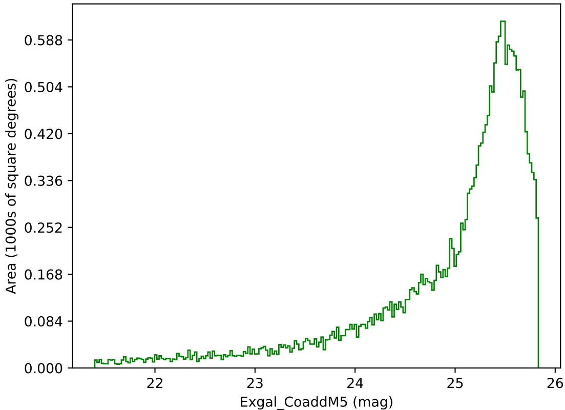
ddf_half_v3.4_10yrs Yr 1 g band: Exgal_CoaddM5
