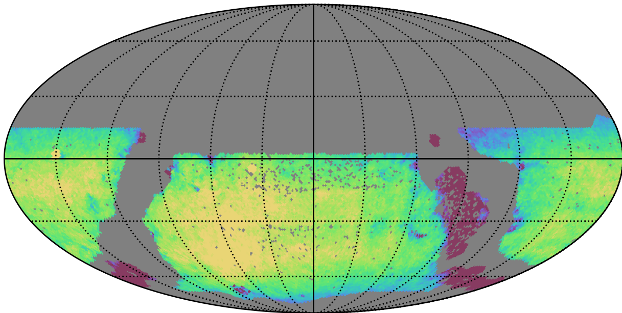
ddf_half_v3.4_10yrs WFD z band: Exgal_CoaddM5
