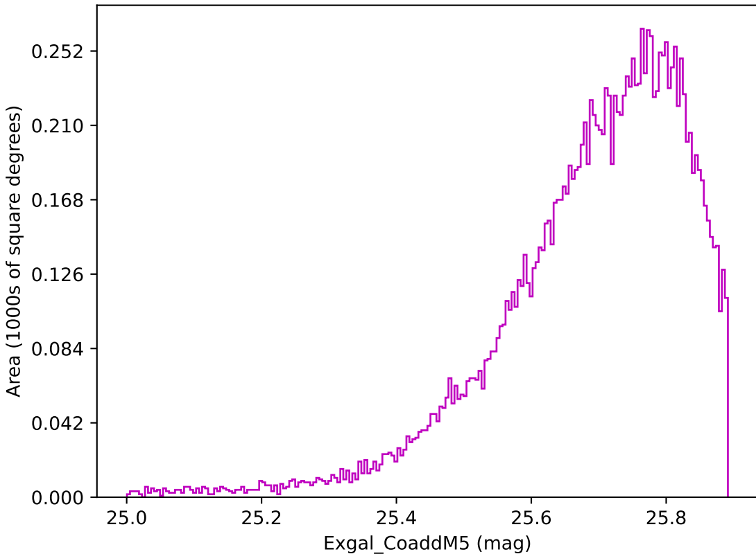
ddf_half_v3.4_10yrs WFD z band: Exgal_CoaddM5
