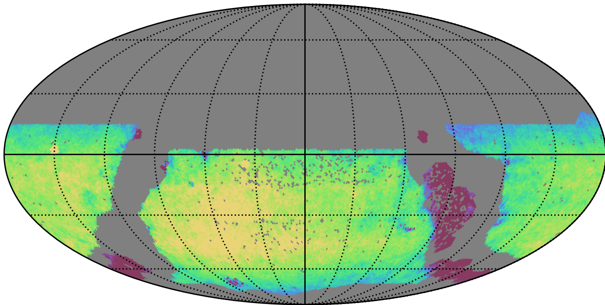
ddf_half_v3.4_10yrs WFD y band: Exgal_CoaddM5
