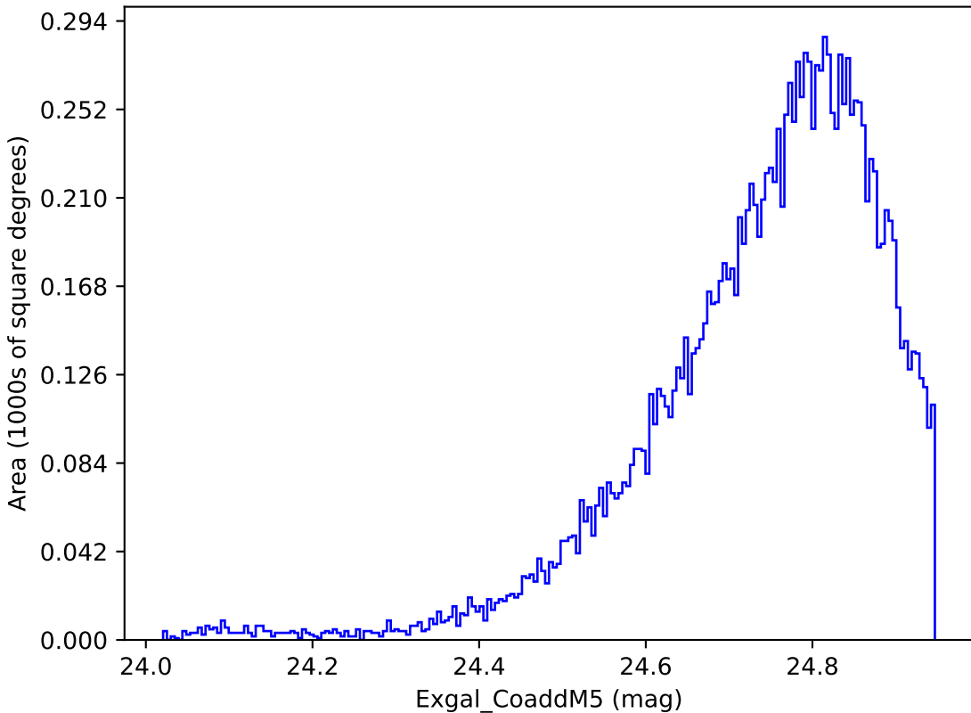
ddf_half_v3.4_10yrs WFD y band: Exgal_CoaddM5
