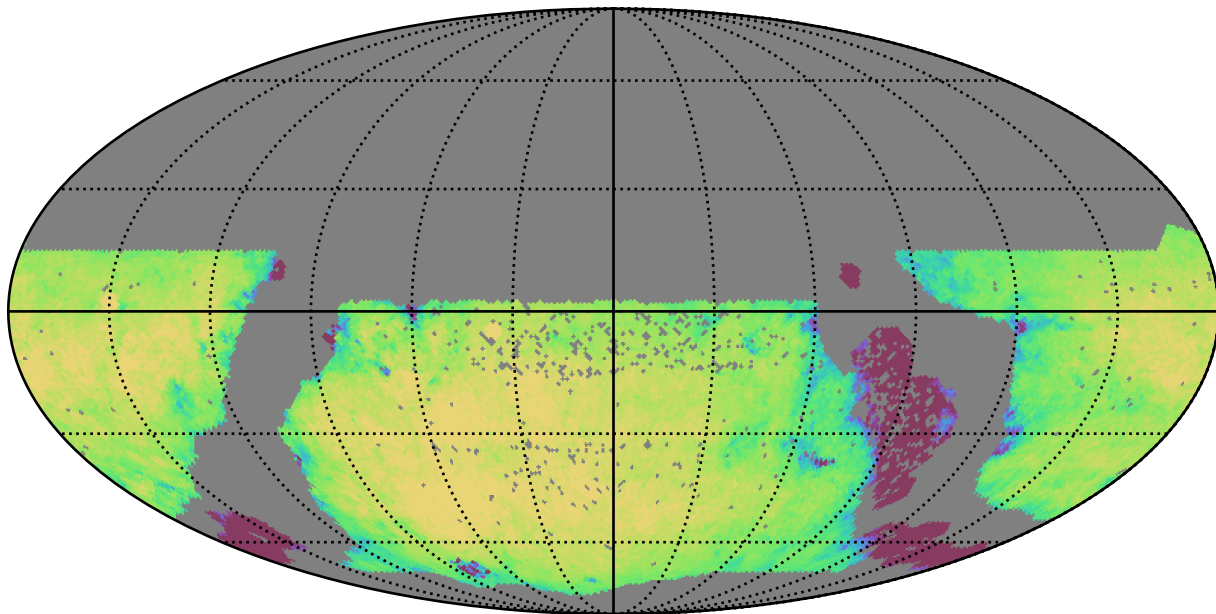
ddf_half_v3.4_10yrs WFD u band: Exgal_CoaddM5
