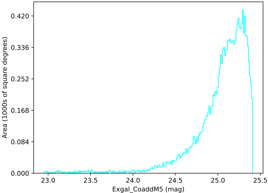
ddf_half_v3.4_10yrs WFD u band: Exgal_CoaddM5
