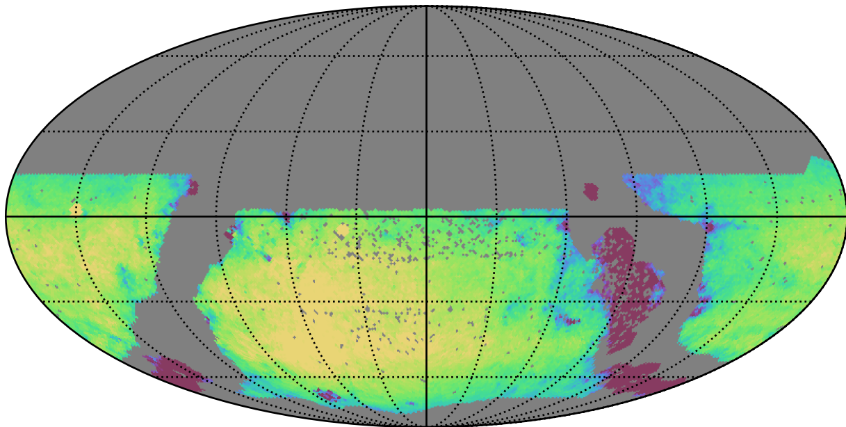
ddf_half_v3.4_10yrs WFD r band: Exgal_CoaddM5
