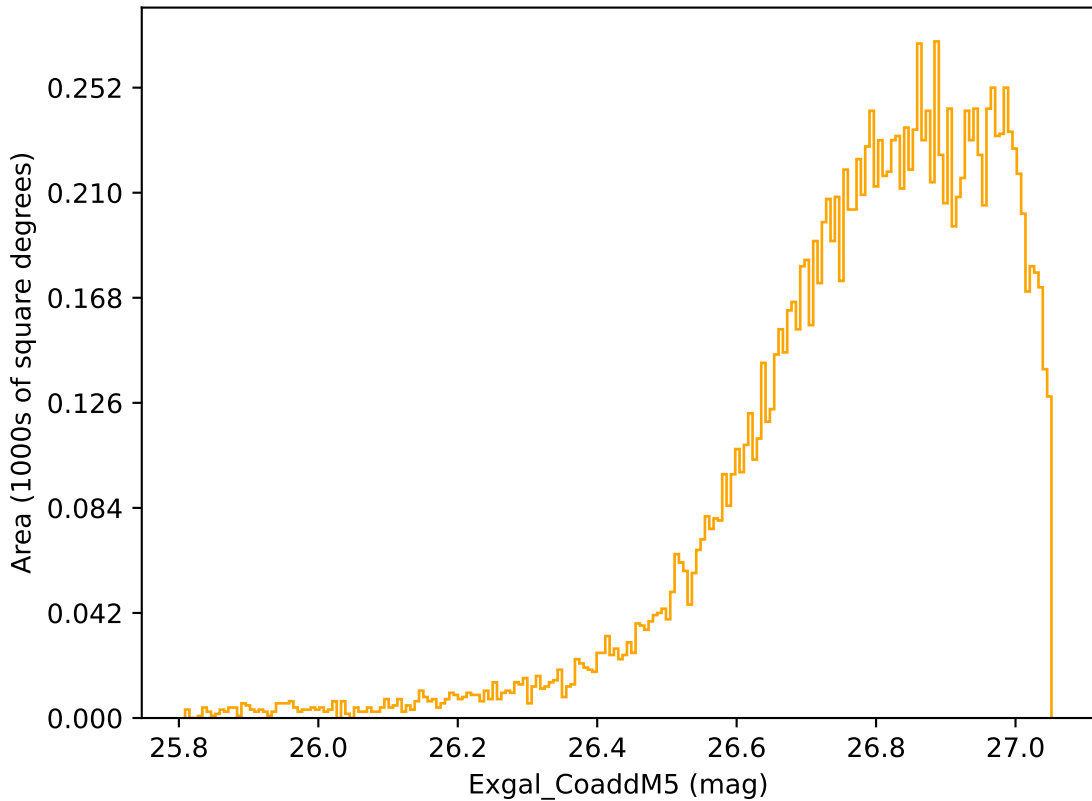
ddf_half_v3.4_10yrs WFD r band: Exgal_CoaddM5
