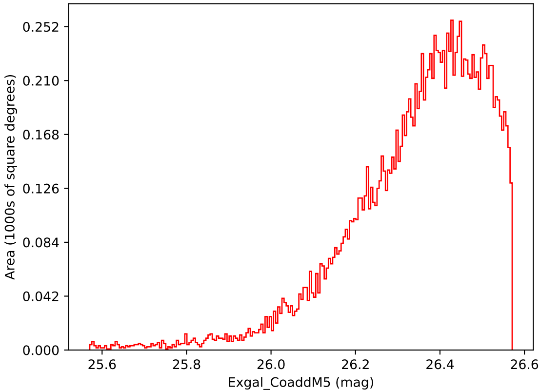
ddf_half_v3.4_10yrs WFD i band: Exgal_CoaddM5
