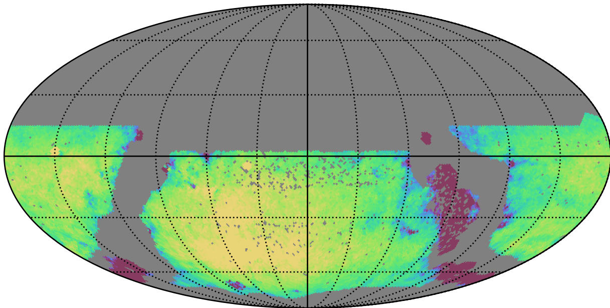
ddf_half_v3.4_10yrs WFD g band: Exgal_CoaddM5
