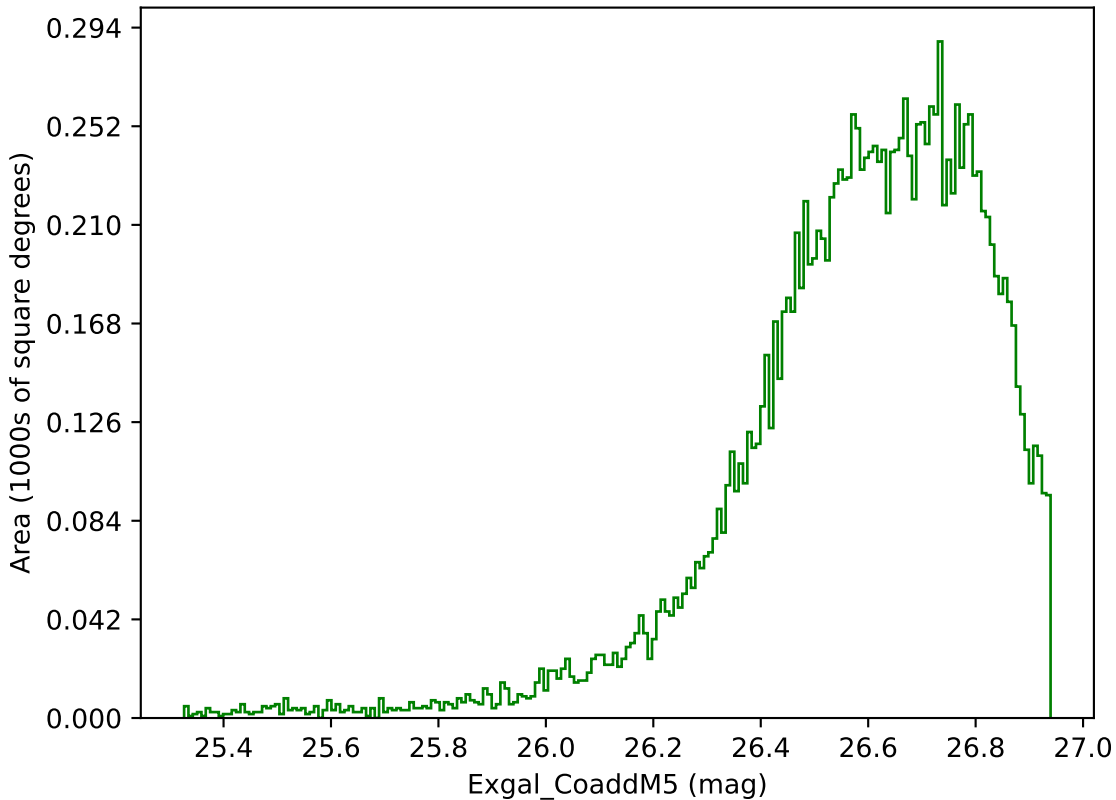
ddf_half_v3.4_10yrs WFD g band: Exgal_CoaddM5
