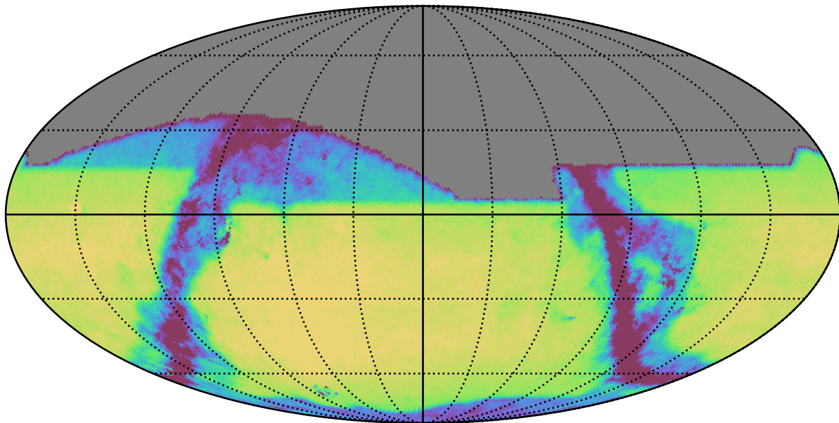
ddf_half_v3.4_10yrs All sky z band: Exgal_CoaddM5
