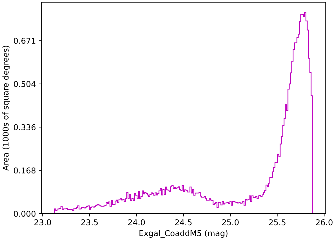
ddf_half_v3.4_10yrs All sky z band: Exgal_CoaddM5
