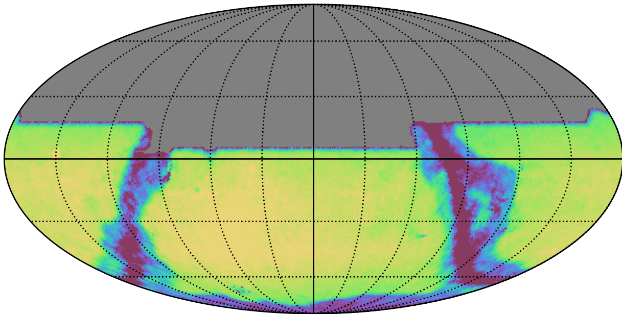
ddf_half_v3.4_10yrs All sky y band: Exgal_CoaddM5
