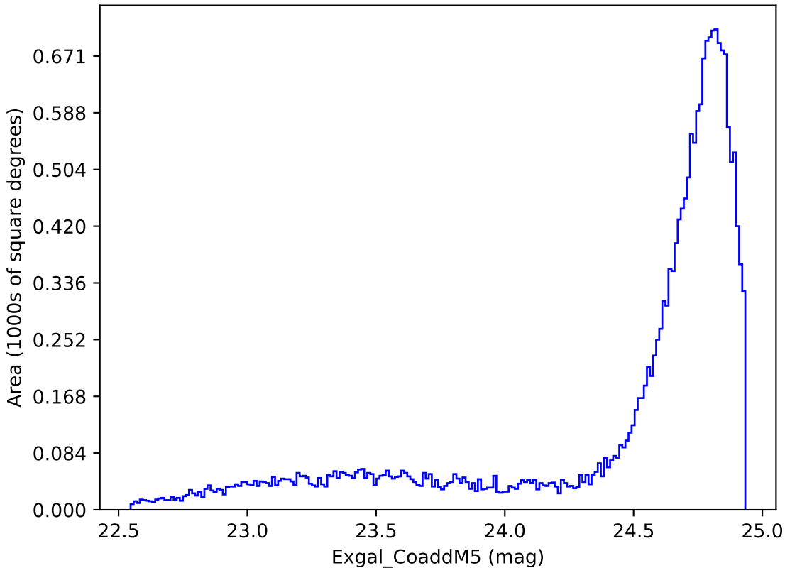
ddf_half_v3.4_10yrs All sky y band: Exgal_CoaddM5
