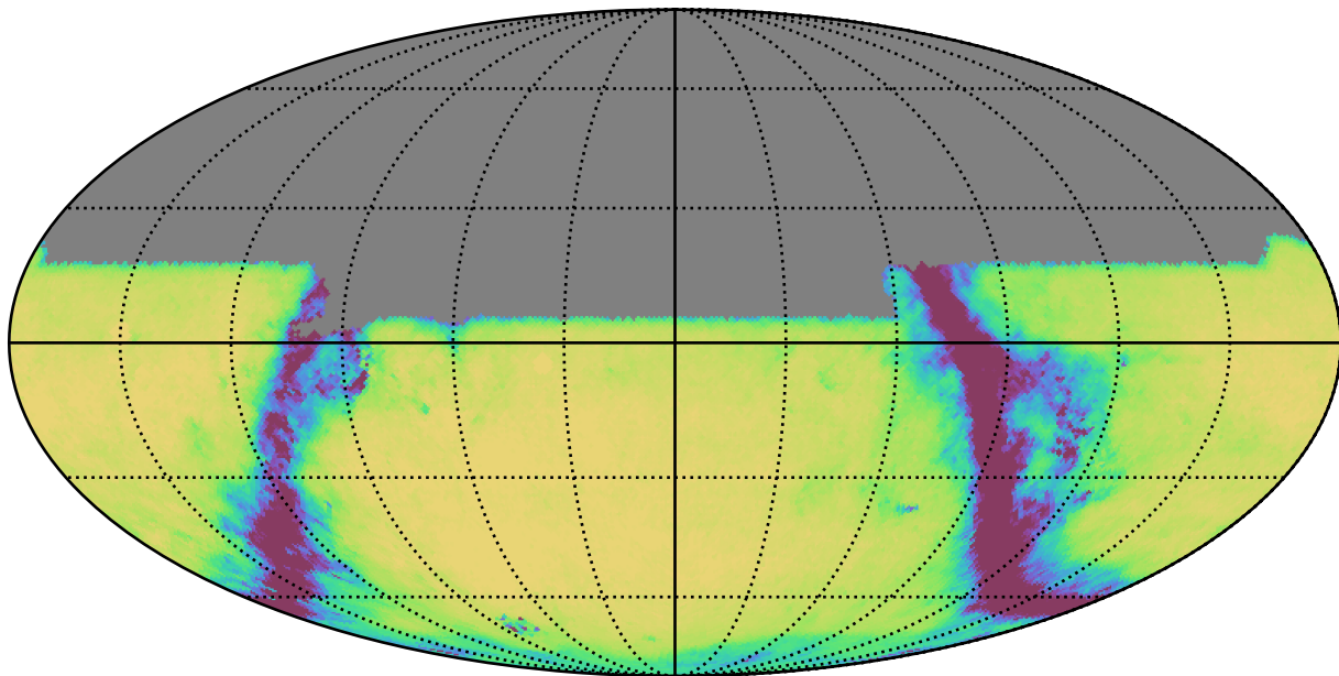
ddf_half_v3.4_10yrs All sky u band: Exgal_CoaddM5
