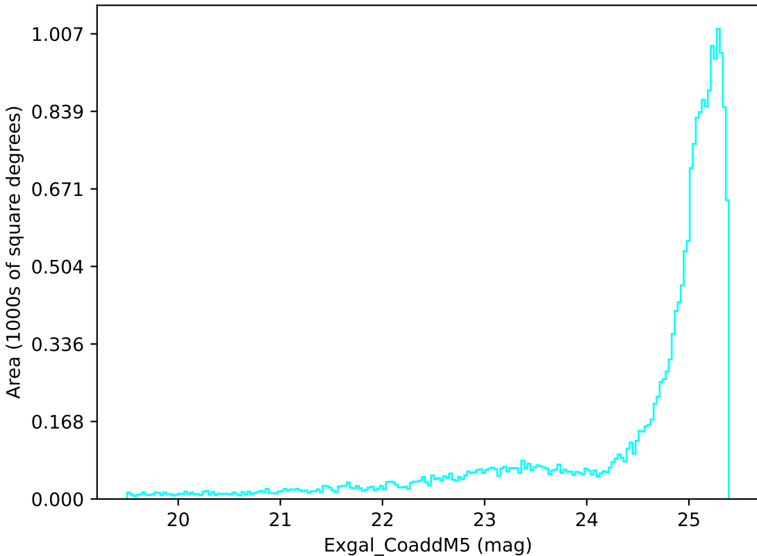
ddf_half_v3.4_10yrs All sky u band: Exgal_CoaddM5
