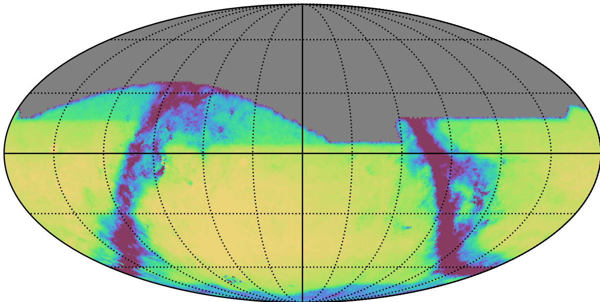
ddf_half_v3.4_10yrs All sky r band: Exgal_CoaddM5
