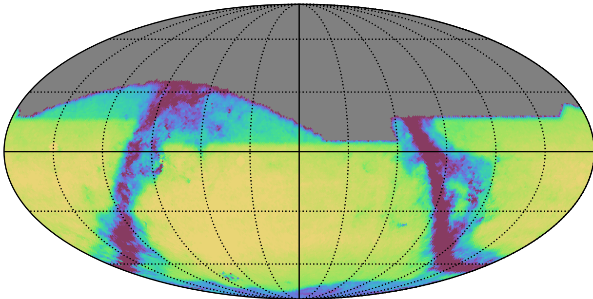
ddf_half_v3.4_10yrs All sky i band: Exgal_CoaddM5
