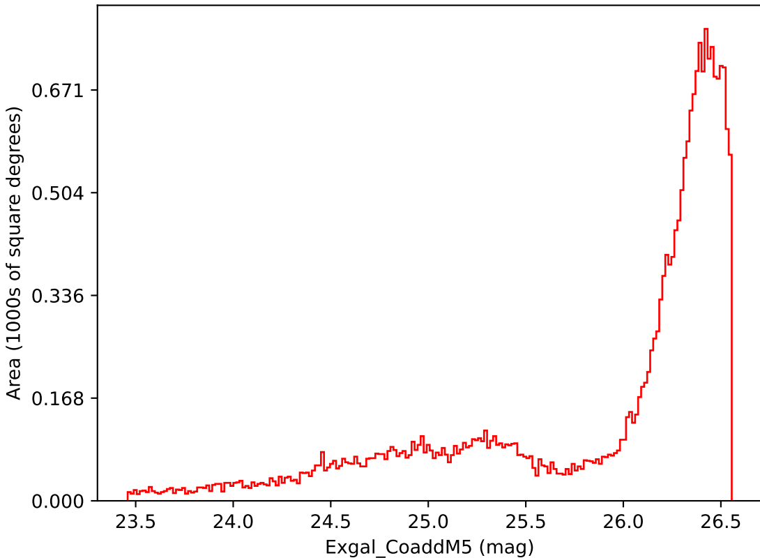
ddf_half_v3.4_10yrs All sky i band: Exgal_CoaddM5
