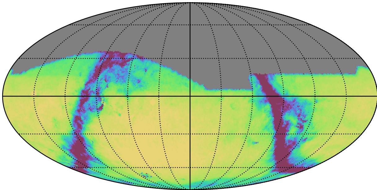
ddf_half_v3.4_10yrs All sky g band: Exgal_CoaddM5
