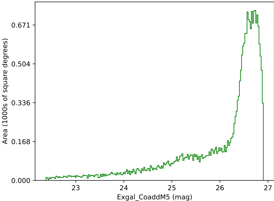
ddf_half_v3.4_10yrs All sky g band: Exgal_CoaddM5
