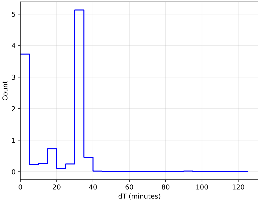
ddf_half_v3.4_10yrs WFD: DeltaT Histogram
