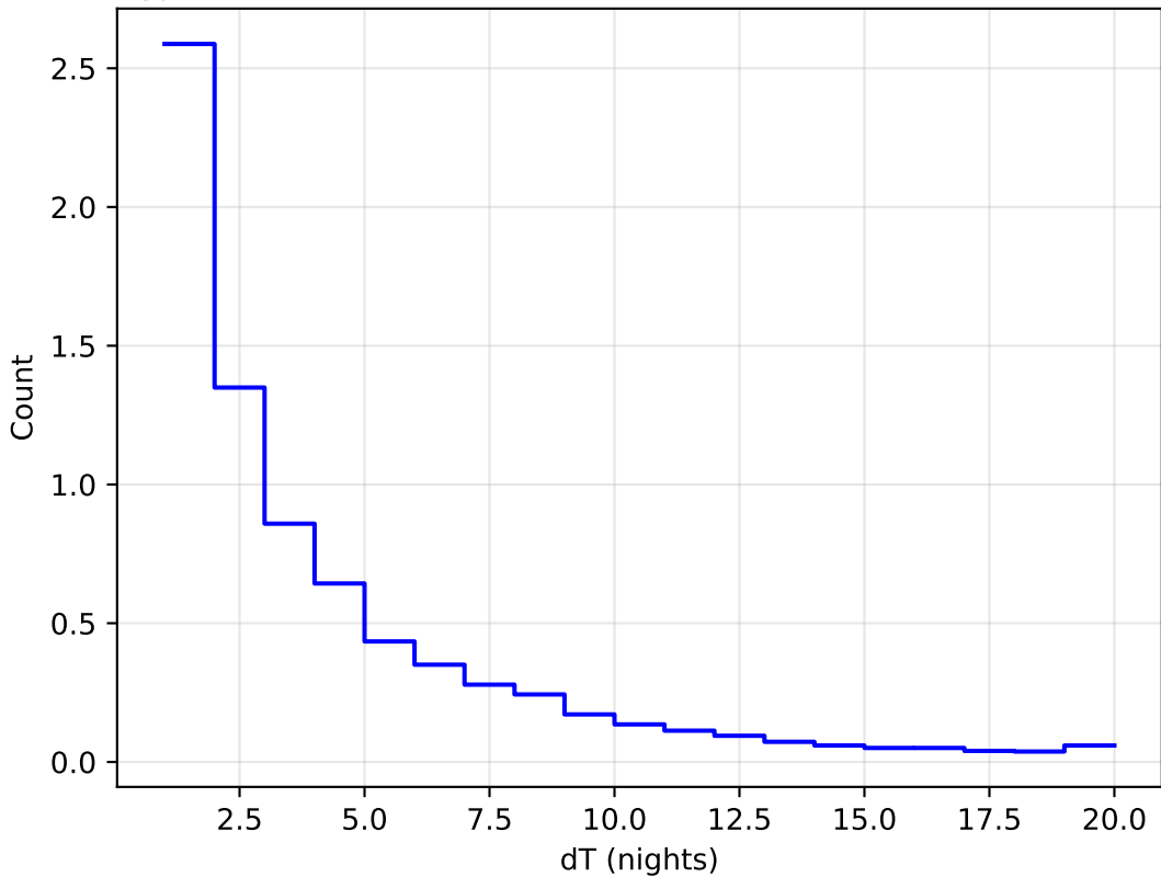
ddf_half_v3.4_10yrs WFD all bands: DeltaNight Histogram 1e6
