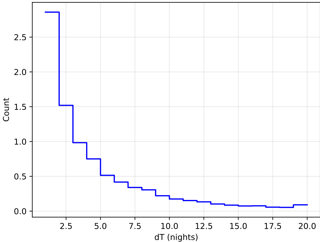
ddf_half_v3.4_10yrs All sky all bands: DeltaNight Histogram 1e6
