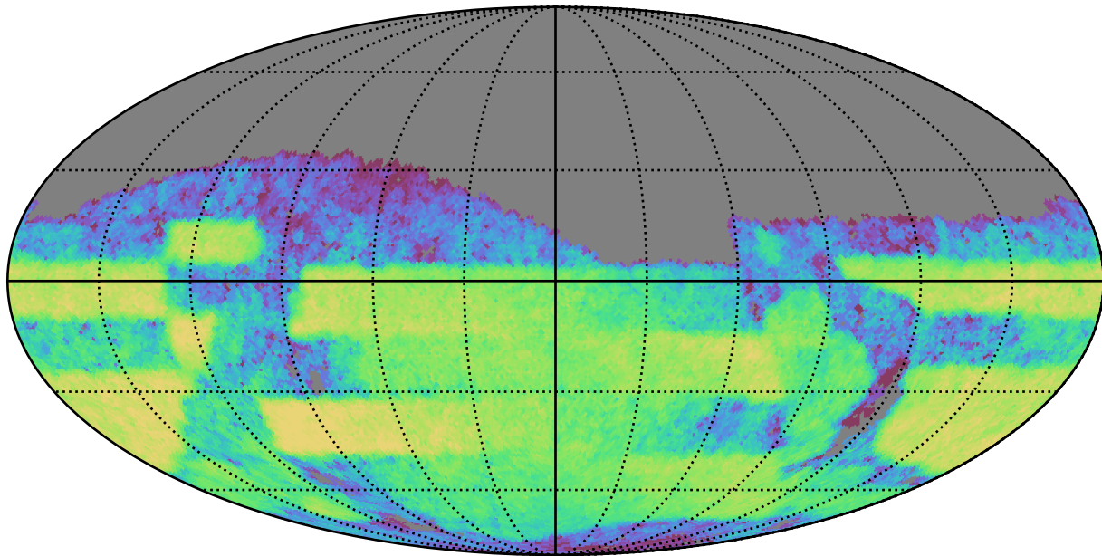
ddf_half_v3.4_10yrs Yr 3-4 z band: CoaddM5
