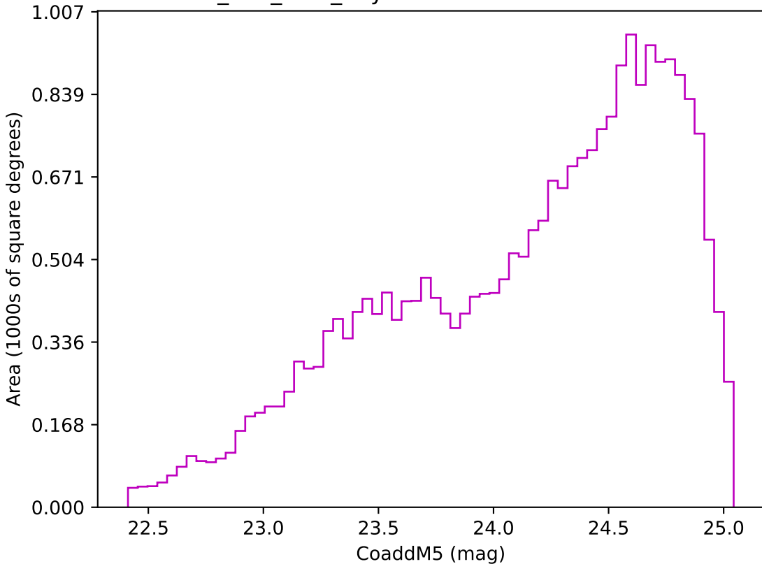
ddf_half_v3.4_10yrs Yr 3-4 z band: CoaddM5
