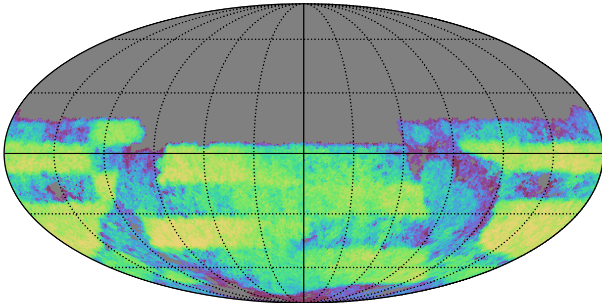
ddf_half_v3.4_10yrs Yr 3-4 y band: CoaddM5
