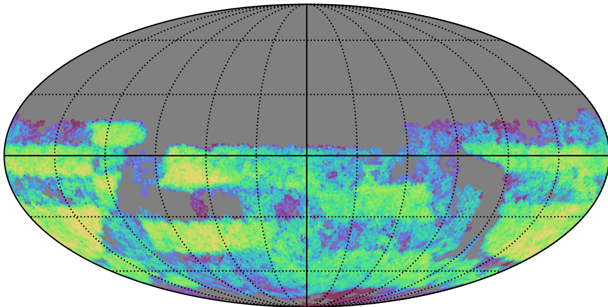
ddf_half_v3.4_10yrs Yr 3-4 u band: CoaddM5
